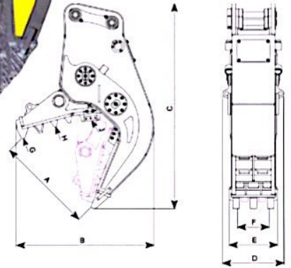
Bolt on type Mounting (B)
