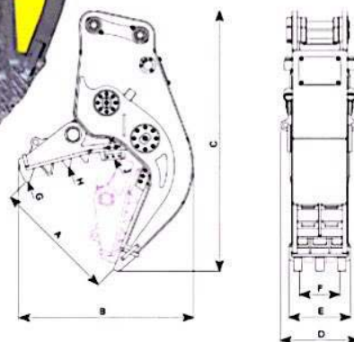
Bolt on type Mounting (B)
