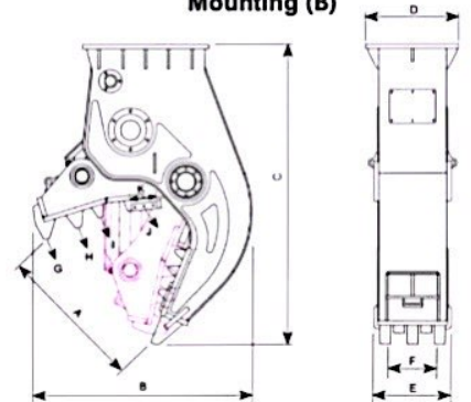
Bolt on type Mounting (B)
